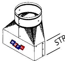
Perimeter Straight Boot 30ga PH-1 Page 12A
